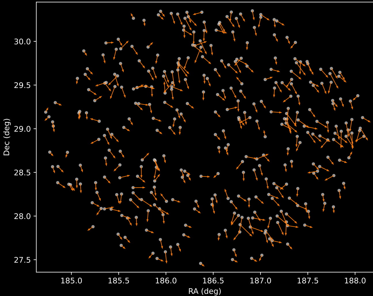
APOGEE DR17 Cluster 2 Proper Motion Vectors (n=339)
