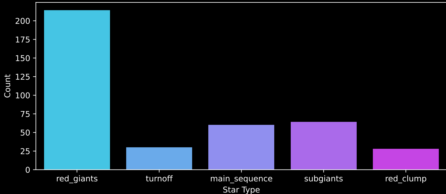
APOGEE DR17 Field: [180+00] Count plot of Star Type
