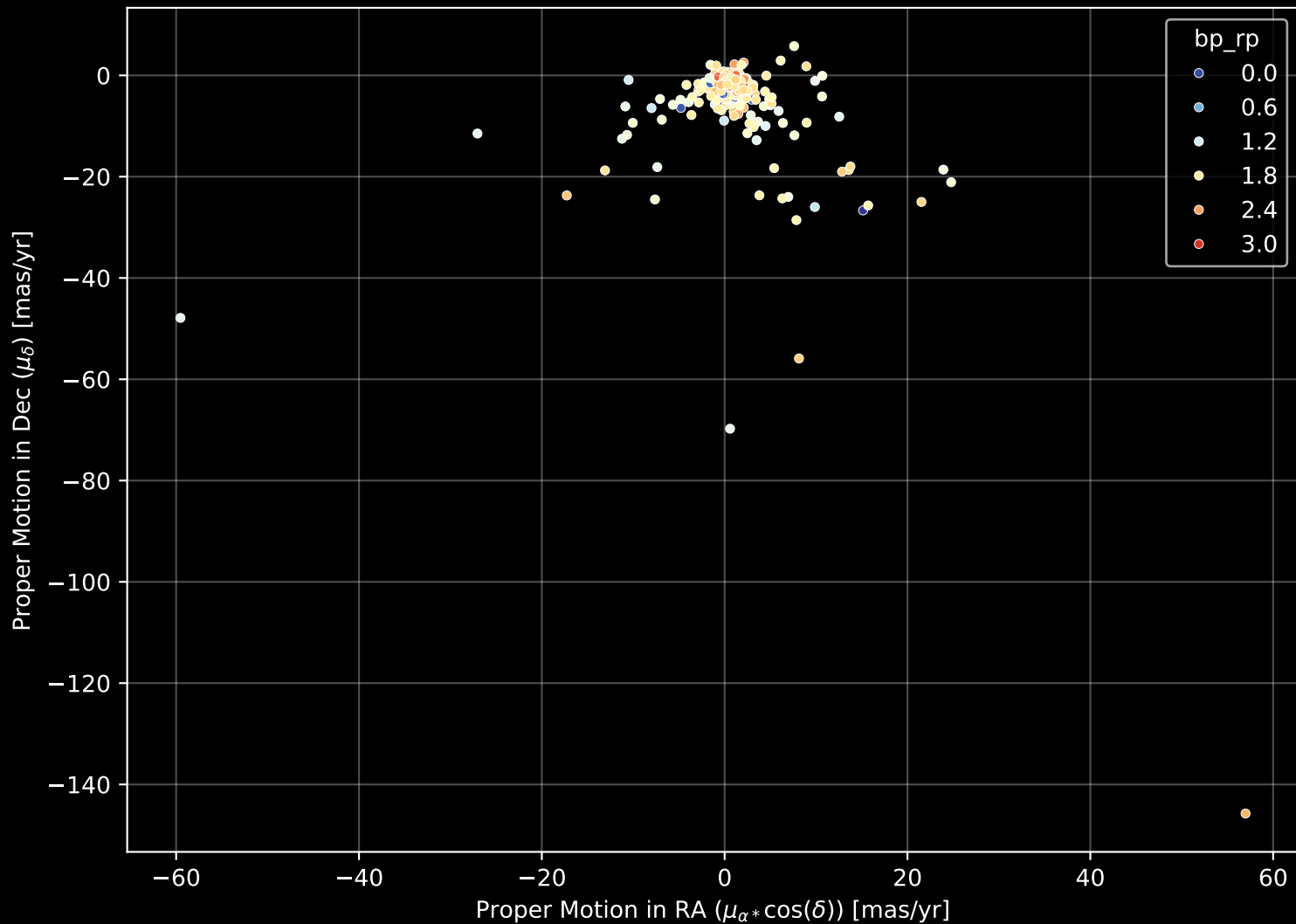
APOGEE DR17 Field: [180+00] Proper Motion Diagram (n= 396)
