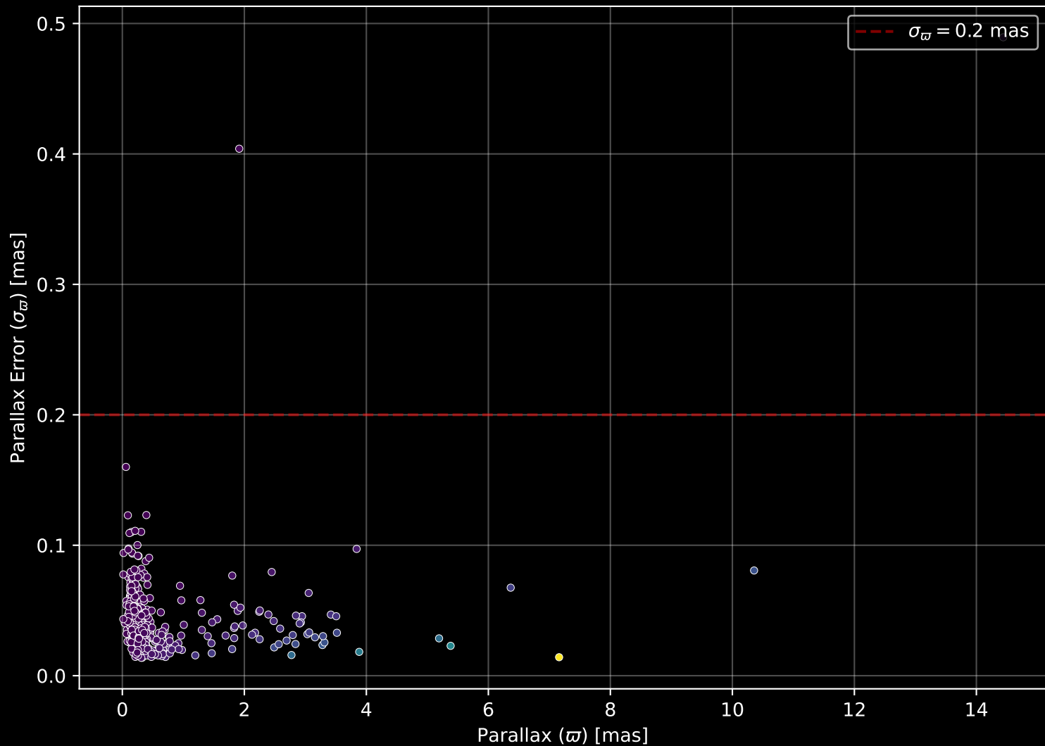
APOGEE DR17 Field: [180+00] Parallax Quality (n= 396)
