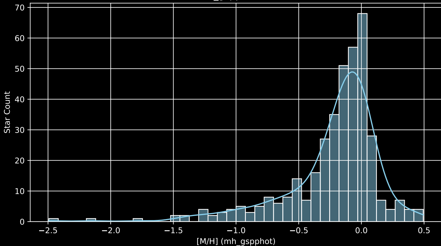
APOGEE DR17 Field: [180+00 [M/H] (mh_gspphot) (n= 384)
