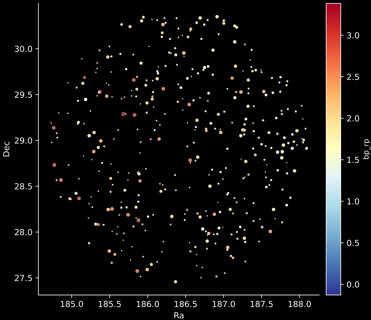
APOGEE DR17 Field: [180+00] Stars: 396
