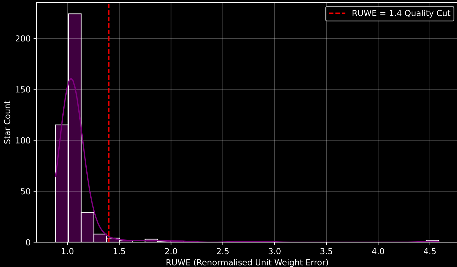
GAPOGEE DR17 Field [180+00] RUWE Distribution (n= 393)
